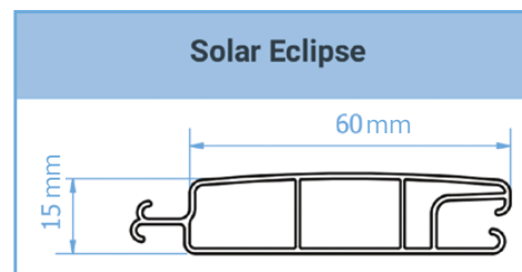
Roldeck Solar Eclipse Lamellen
